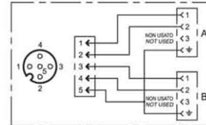
CONNECTOR M12x1 CONNECTION SCHEME
